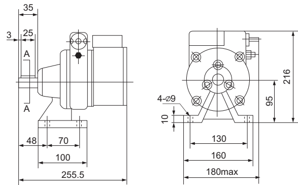
LLY1-3S/□型超速开关外形及安装尺寸 LLY1-3S/□ overspeed switch shape and mounting dimensions
