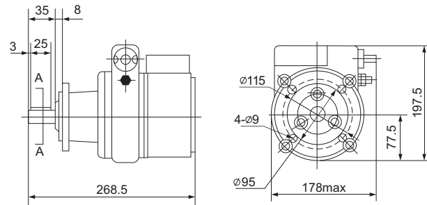
LLY1-3S/□D型超速开关外形及安装尺寸 LLY1-3S/□D overspeed switch shape and mounting dimensions
