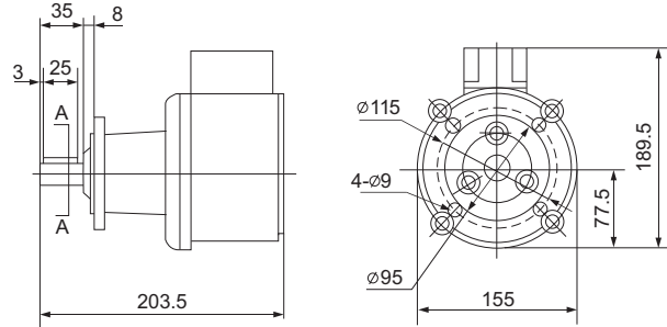
LLY1-2/□D型超速开关外形及安装尺寸 LLY1-2/□D overspeed switch shape and mounting dimensions
